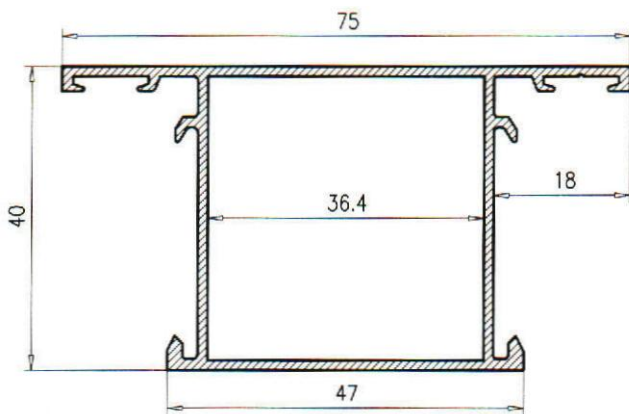
Pilastra 40*40 09
