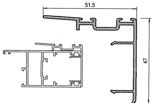
Clip Central 615
