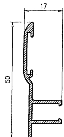
Acople 3 carriles 620
