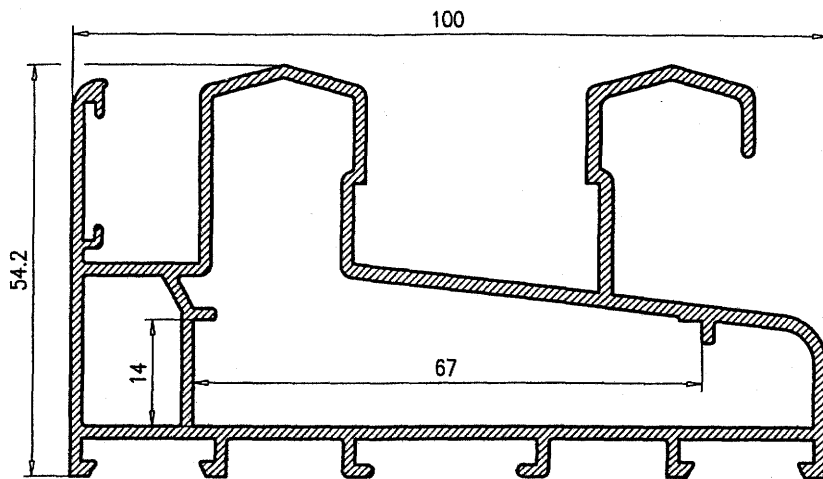
Marco Perimetral 100 614
