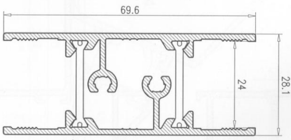
Parteluz Climalit PRT 17001
