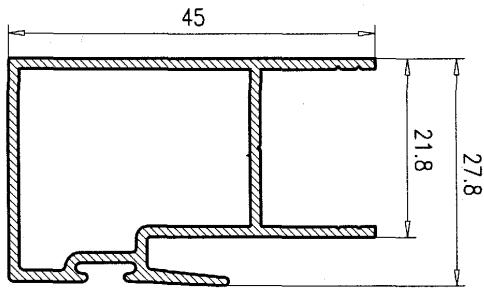
Hoja Central Climalit 45 7015
