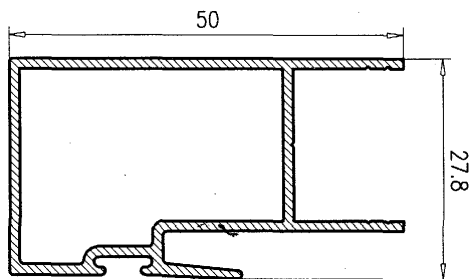
Hoja Central Climalit 50 7013
