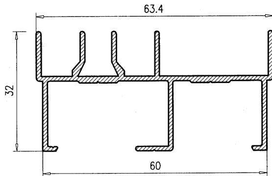
Marco Lateral 7028
