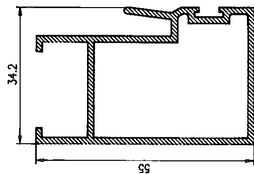
Hoja Central Climalit 55 124341
