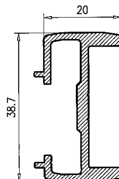
Marco Lateral 62
