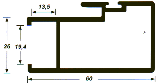
Hoja Central Climalit 7213
