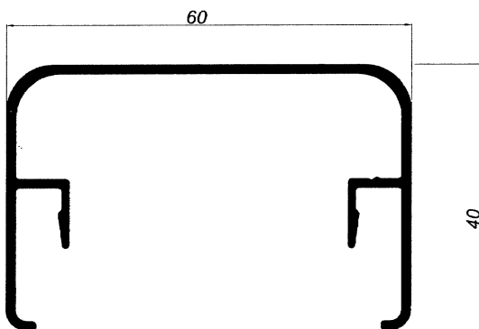
Pasamano Rectangular 60*40 326
