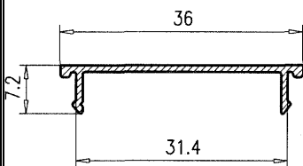
Grapa 800
