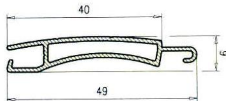
Lama Persiana 40 7932
