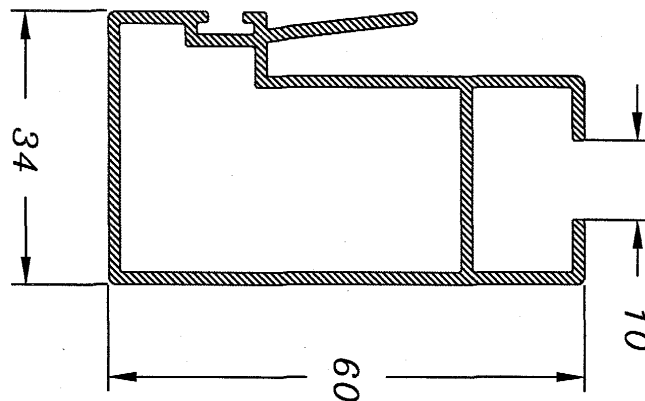
Hoja Central Normal 95
