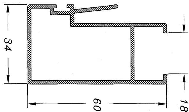
Hoja Central Climalit 99
